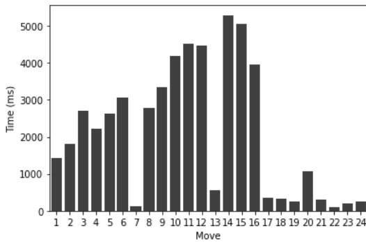
Fig. 4. Minmax bar graph for 1 game
