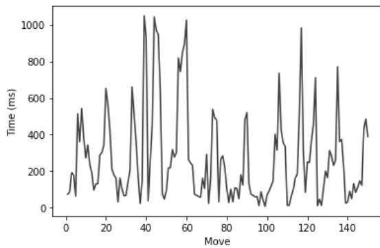
Fig. 8. 5.Minmax line graph plot for 10 games
