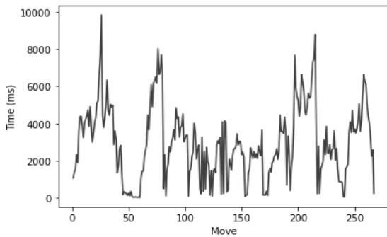
Fig. 5. Minmax line graph plot for 10 games
