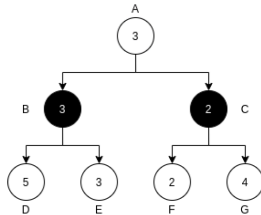
Fig. 2. Ex. Game tree with -\beta pruning
