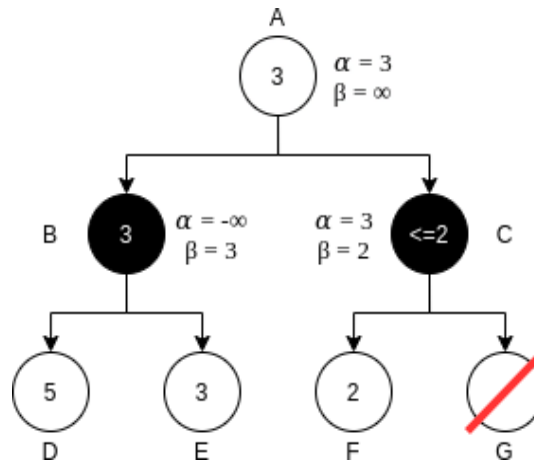
Fig. 3. Ex. -\beta pruning
