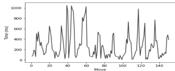
Fig. 7. 4.Minmax with alpha-beta bar graph plot for 1 game
